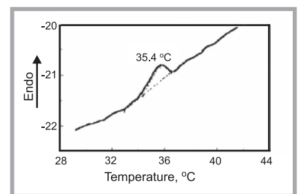
Figure 7. DSC curves of PNIPAAm-g-cotton in wet condition [18].
