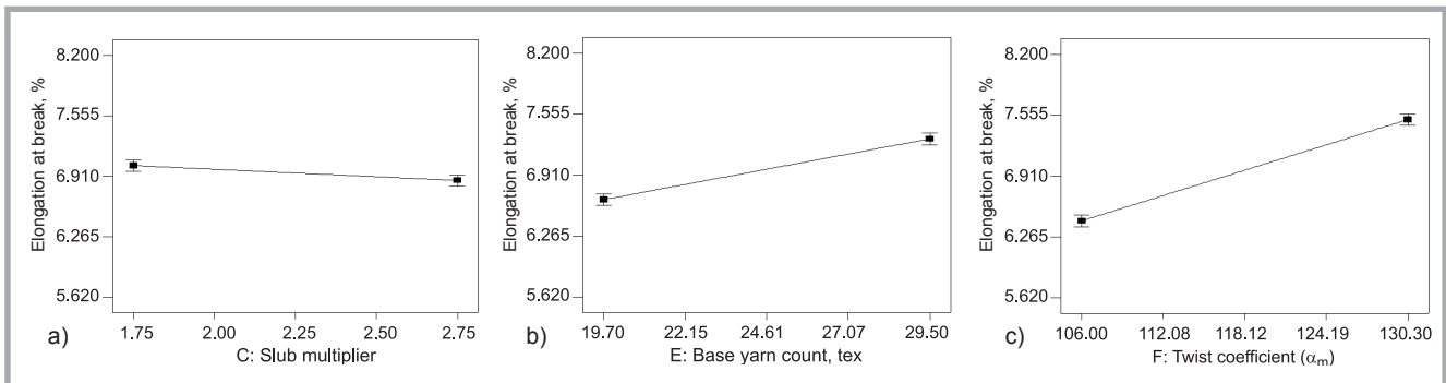
Figure 7. Main effect plots of significant factors for the breaking elongation.
