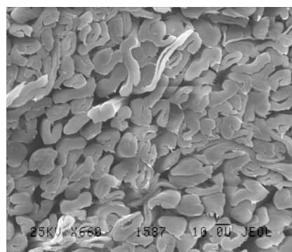
Figure 10. Microscopic pictures of fibre cross-sections of cottons containing the smallest number of immature fibres: a) Turkish brown (TB), b) Turkish light brown short (TLBS).
