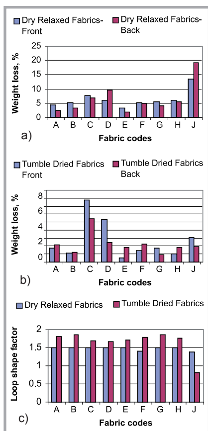
Figure 1. Pile losses and loop shape of the particular fabrics; a) pile loss on dry-relaxed fabrics after abrasion, b) pile loss on tumble-dried fabrics after abrasion, c) loop shape factor of fabrics.
