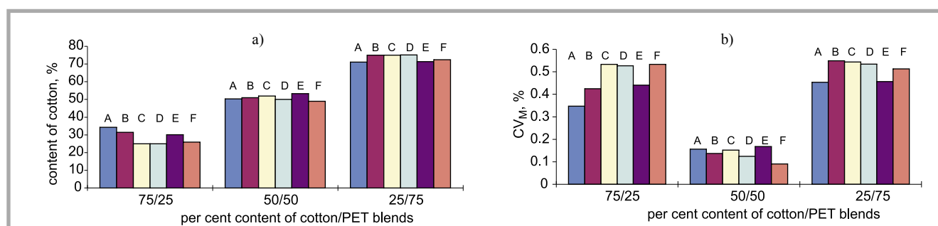
Figure 1. Real percentage content of cotton in the blend (a), and coefficients of variation of the fibre blends (b); A) cotton ring-spun carded, B) cotton ring-spun combed, C) cotton rotor-spun (BD-200S) carded, D) cotton rotor-spun (BD-200S) combed, E) cotton rotor-spun (R1) carded, F) cotton rotor-spun (R1) combed.
