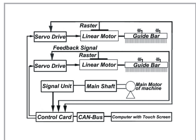
Figure 1. Principle of electric Shogging control system on High speed warp knitting machine.
