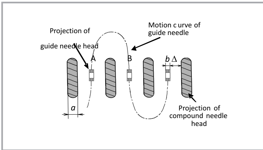
Figure 3. The sketch of the motion curve of the guide needle (laps 1 needle).
