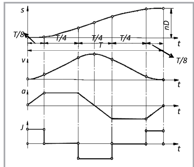
Figure 2. The motion rule of trapezoidal acceleration curve.
