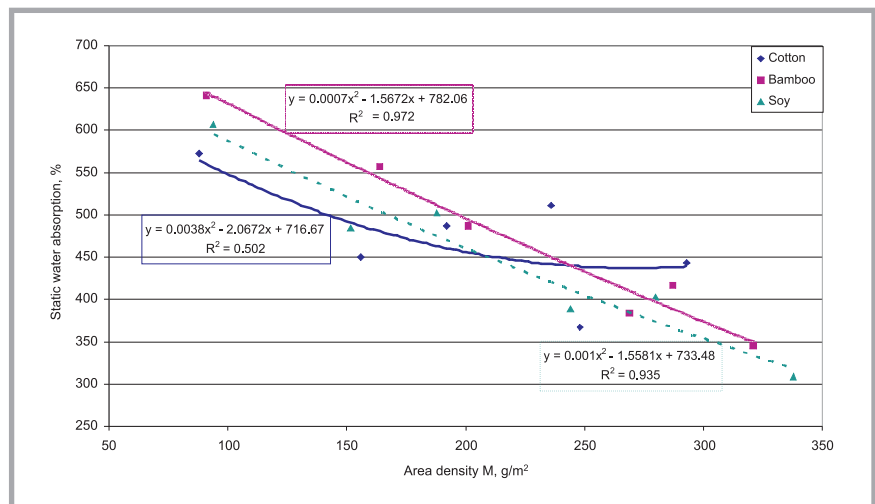
Figure 4. Static water absorption as the function of area density of all cotton (◆), bamboo (■), soy (▲) knits variants.
