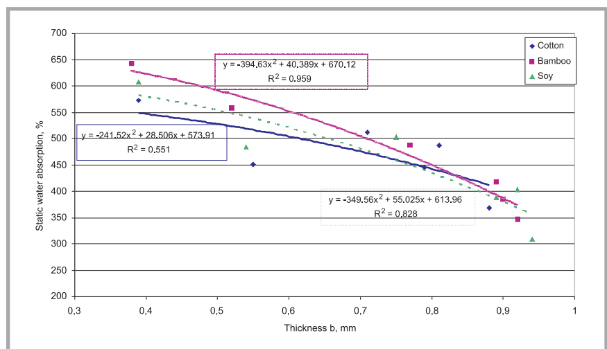
Figure 5. Static water absorption as the function of thickness of all cotton (◆), bamboo (■), soy (▲) knits variants.
