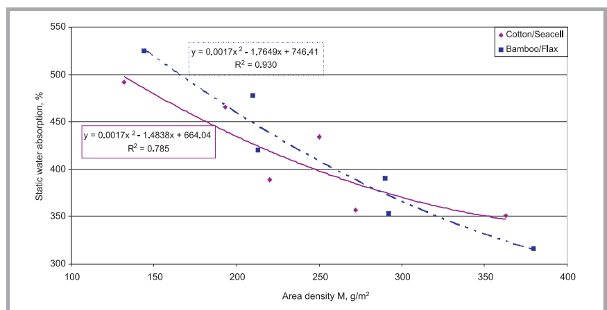
Figure 6. Static water absorption as the function of area density of all cotton/seacell (◆), bambo/flax (■), knits variants.
