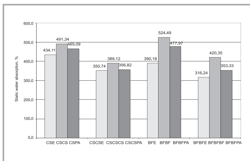
Figure 3. Static water absorption of knits manufactured from Cotton – seacell (CSCS-38 tex, CSCSCS-57 tex), combination with elastane (CSE-29 tex, CSCSE-48 tex) and textured polyamide (CSPA-39 tex, CSCSPA-58tex); Bamboo – flax (BFBF-48 tex, BFBFBF-72 tex), combination with elastane (BFE-34 tex, BFBFE-58 tex) and textured polyamide (BFFA-44 tex, BFBFPA-68 tex) threads.
