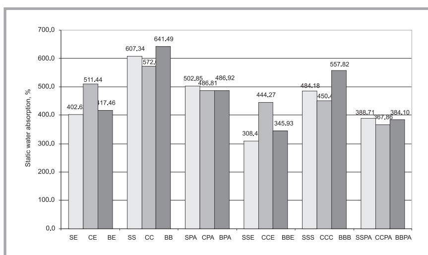
Figure 2. Static water absorption of pure knits manufactured from soy, cotton, bamboo (linear density XX-28 tex, XXX-42 tex) and its combination with elastane (XE-24 tex, XXE-38 tex) and textured polyamide (XPA-34tex, XXPA-48 tex) threads.
