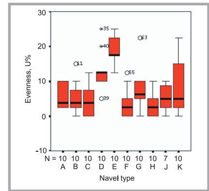
Figure 4. Box-plot diagram showing influence of navel properties on 49-tex rotor yarn evenness (U%).
