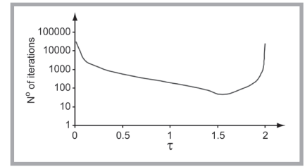
Figure 2. Number of iterations vs. \tau , 4\sqrt{2} \times 4\sqrt{2}l^2 , \epsilon = 10^{-9} .
