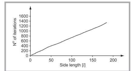
Figure 4. Minimum number of iterations vs. sheet size, \epsilon = 10^{-9} .
