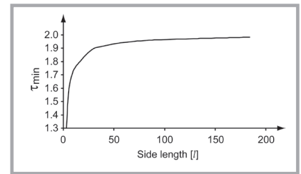
Figure 3. \tau_{min} vs. sheet size, \epsilon = 10^{-9} .
