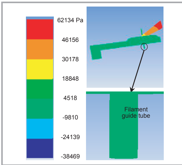
Figure 2. Static pressure in spinning unit.
