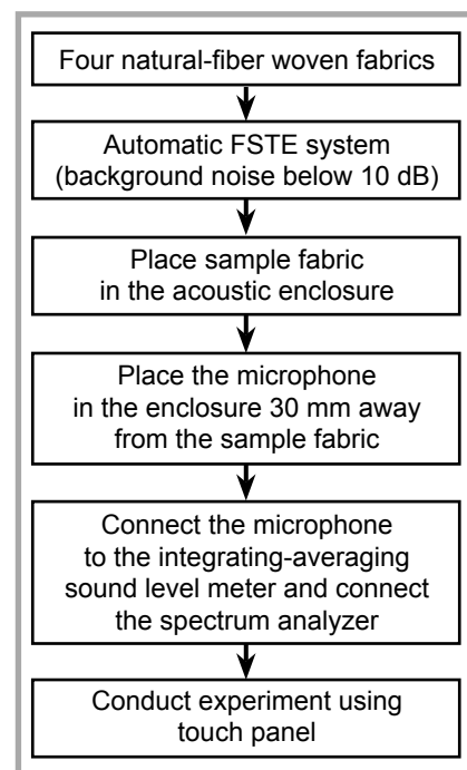
Figure 2. Flow chart of the automatic FSTE system [12-17].
