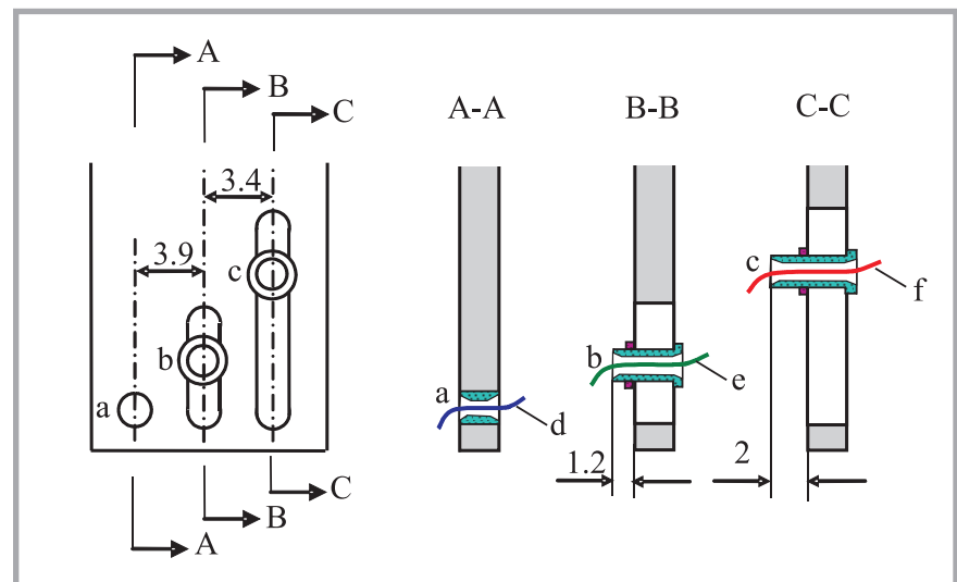
Figure 2. Configuration of the yarn carrier.
