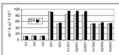
Figure 7. The thermal resistance of the textile materials.
