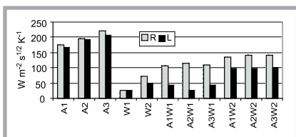
Figure 6. The thermal absorption of the textile materials.
