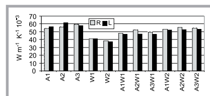
Figure 2. The thermal conductivity of the textile materials.
