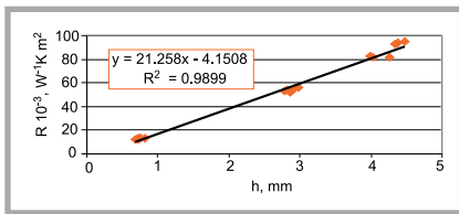
Figure 8. Relationship between the thickness of the textile materials and their thermal resistance.
