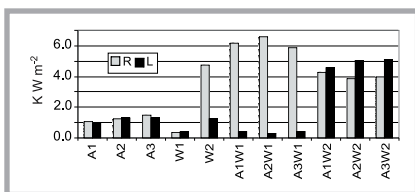
Figure 11. The maximum heat flow density.
