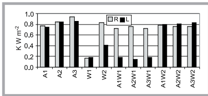
Figure 9. The stationary heat flow density.
