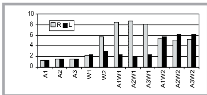
Figure 10. The ratio of the maximum and stationary heat flow density.
