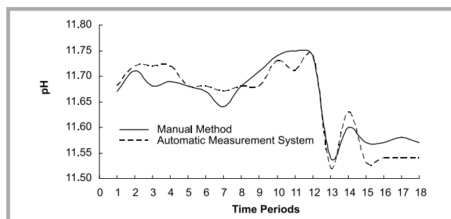
Figure 7. pH measurements of the dye bath with manual method and automatic measurement system.
