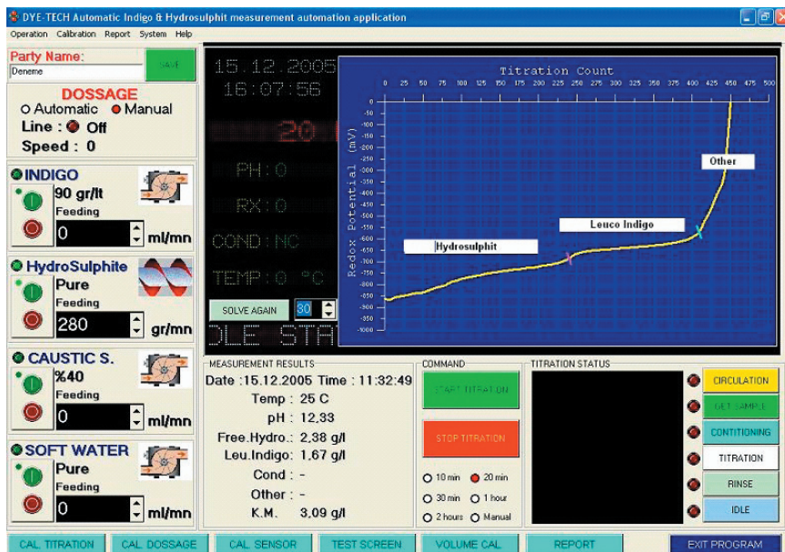
Figure 3. View of the control panel with screen and an example of titration curve.
