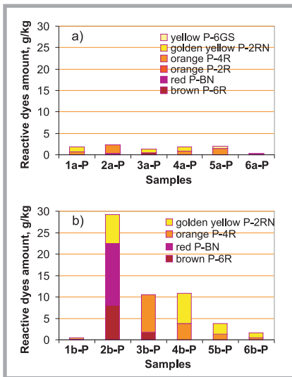
Figure 6. Amount of reactive dyes in the colour printing pastes for rotary screen printing process for design 'a' (a) and design 'b' (b).
